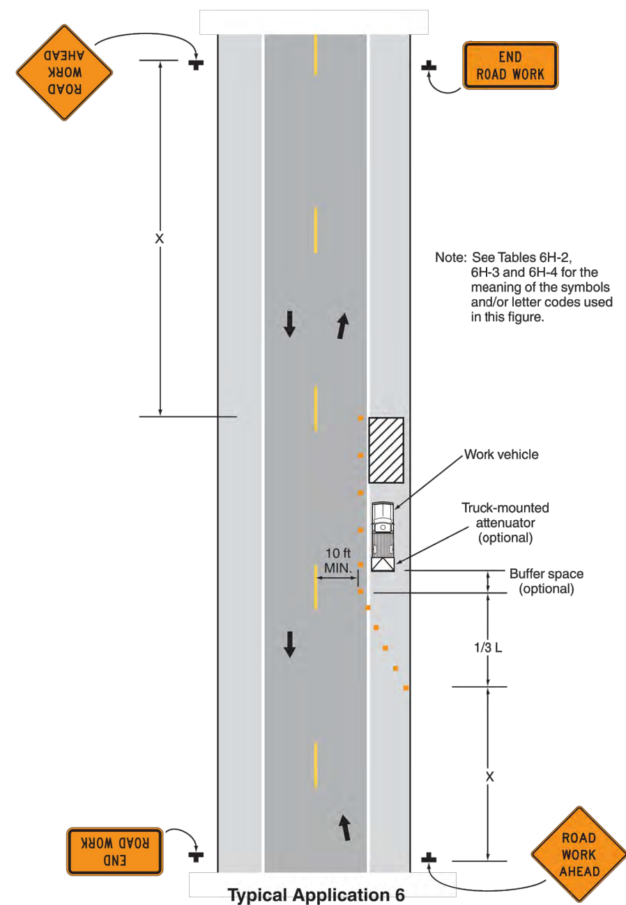
Figure 6H-6. Shoulder Work with Minor Encroachment (TA-6)
