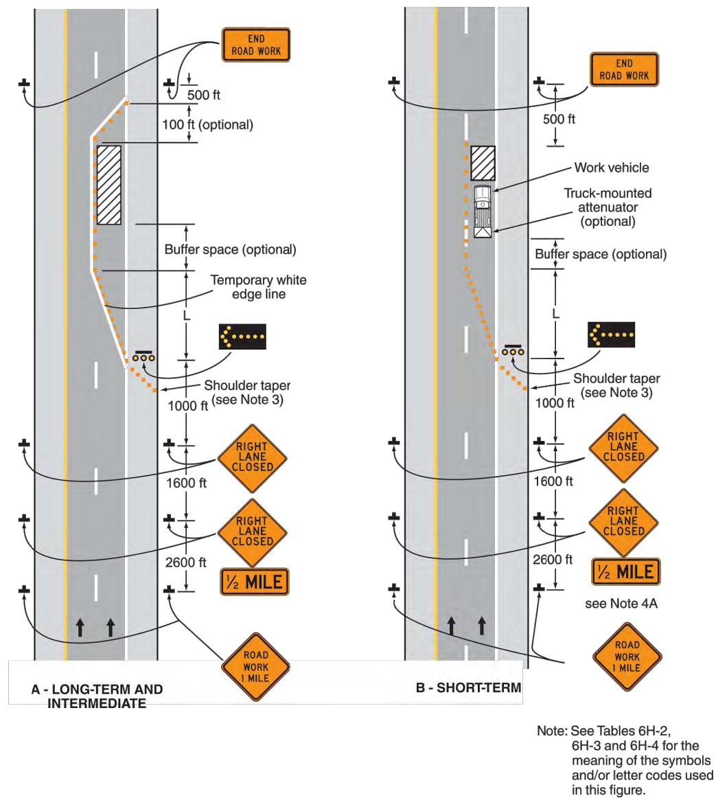
Typical Application 33
