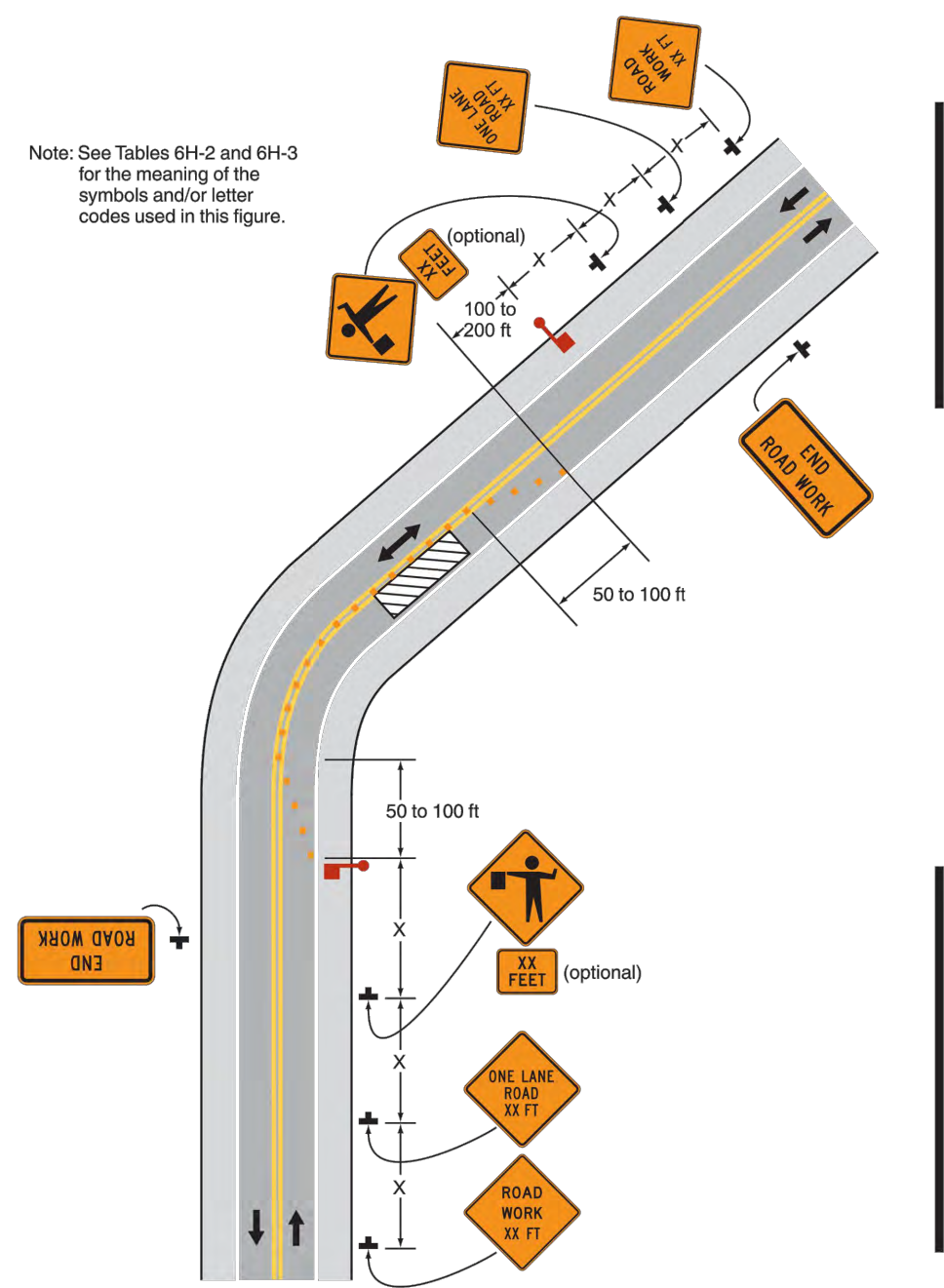
Typical Application 10
