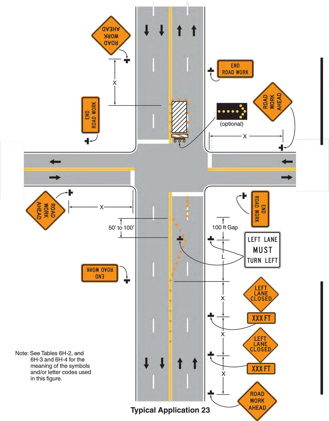
Figure 6H-23. Left-Hand Lane Closure on the Far Side of an Intersection (TA-23)
